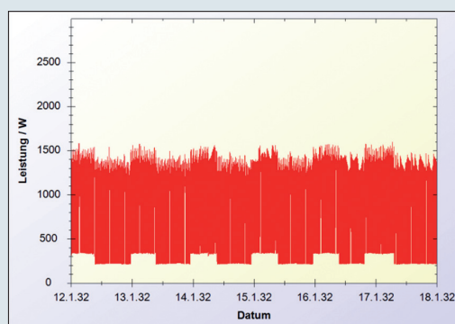
Abb. 71. Lastgang Woche, H18M01
