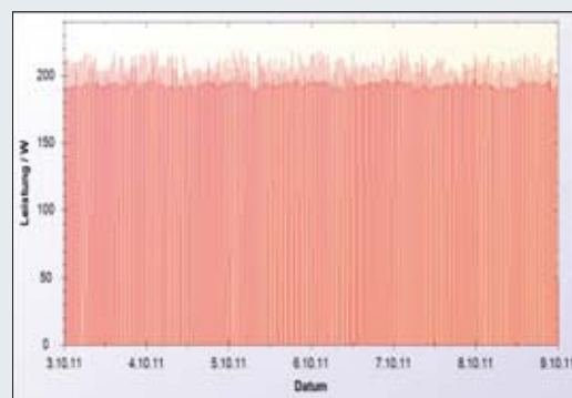
Abb. 85. Lastgang Woche, H15M04
